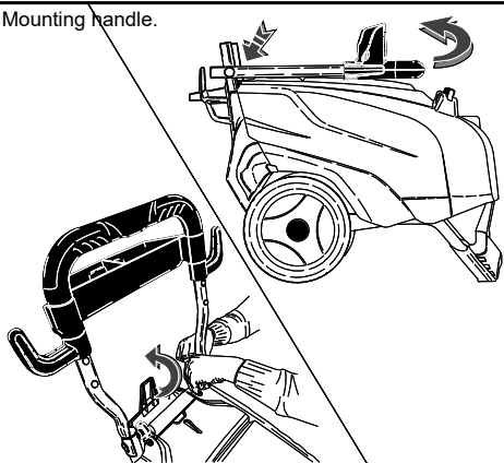
Mounting handle.
