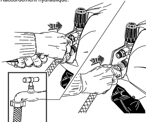
Raccordement hydraulique.
