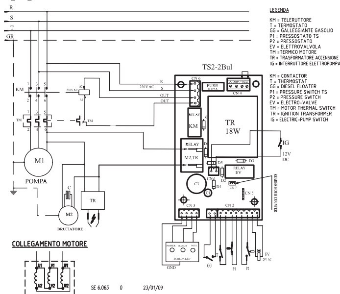
LP_3Ph_220V
